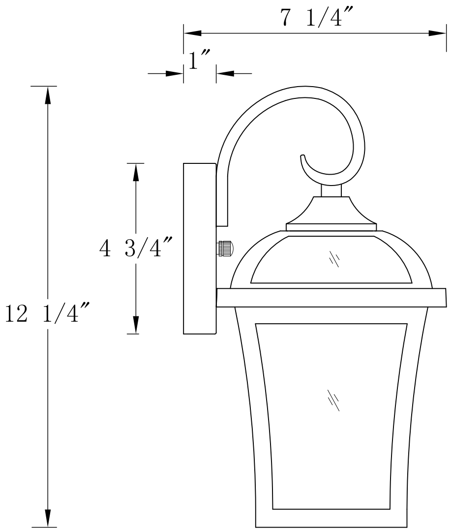
SIDE VIEW
