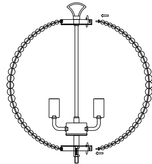
STEP 4 Secure all the wood bead branches.
