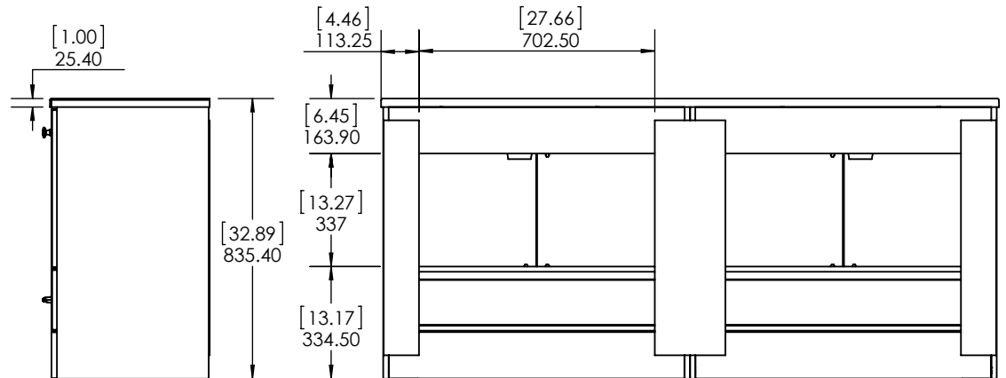
BACK VIEW
