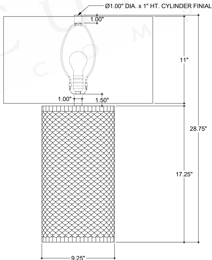
FRONT VIEW
