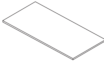
E -600X322X5mm(1pc)
