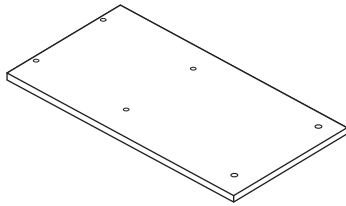
A -600X340X12mm(1pc)
