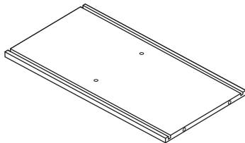
B -600X338X12mm(1pc)
