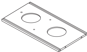
C -600X338X12mm(1pc)
