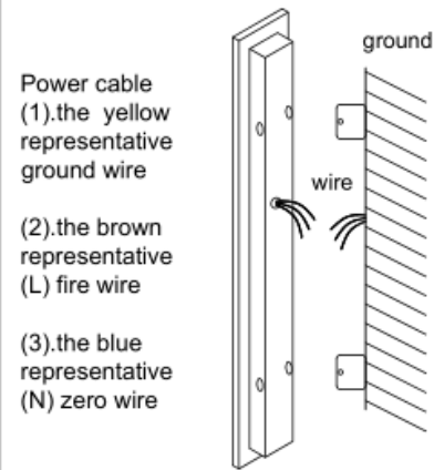
3 Connect the power cord
