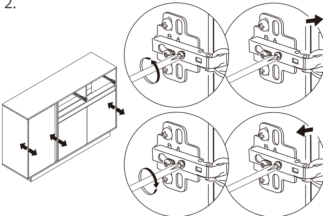
Hinge Lateral Adjustment (Left/Right)
