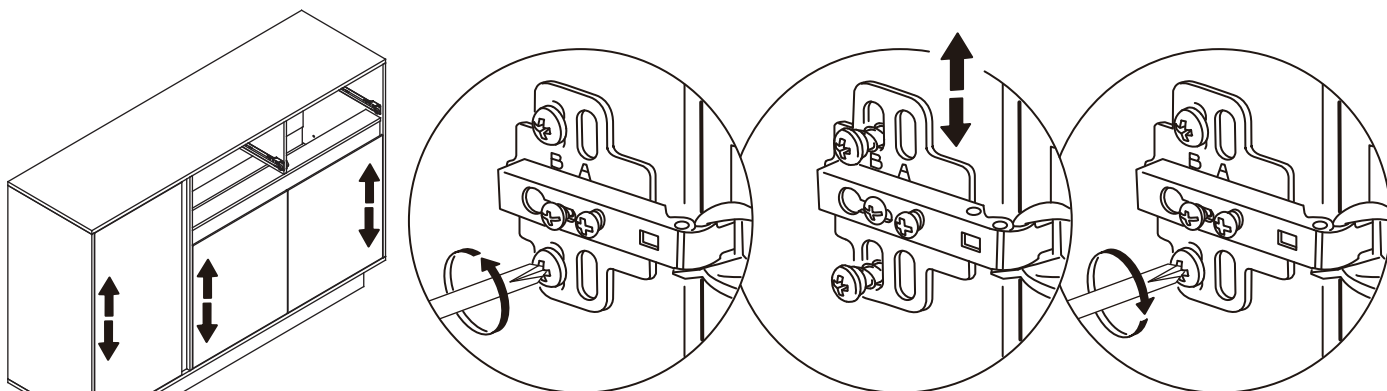
Hinge Vertical Adjustment (Up/Down)
