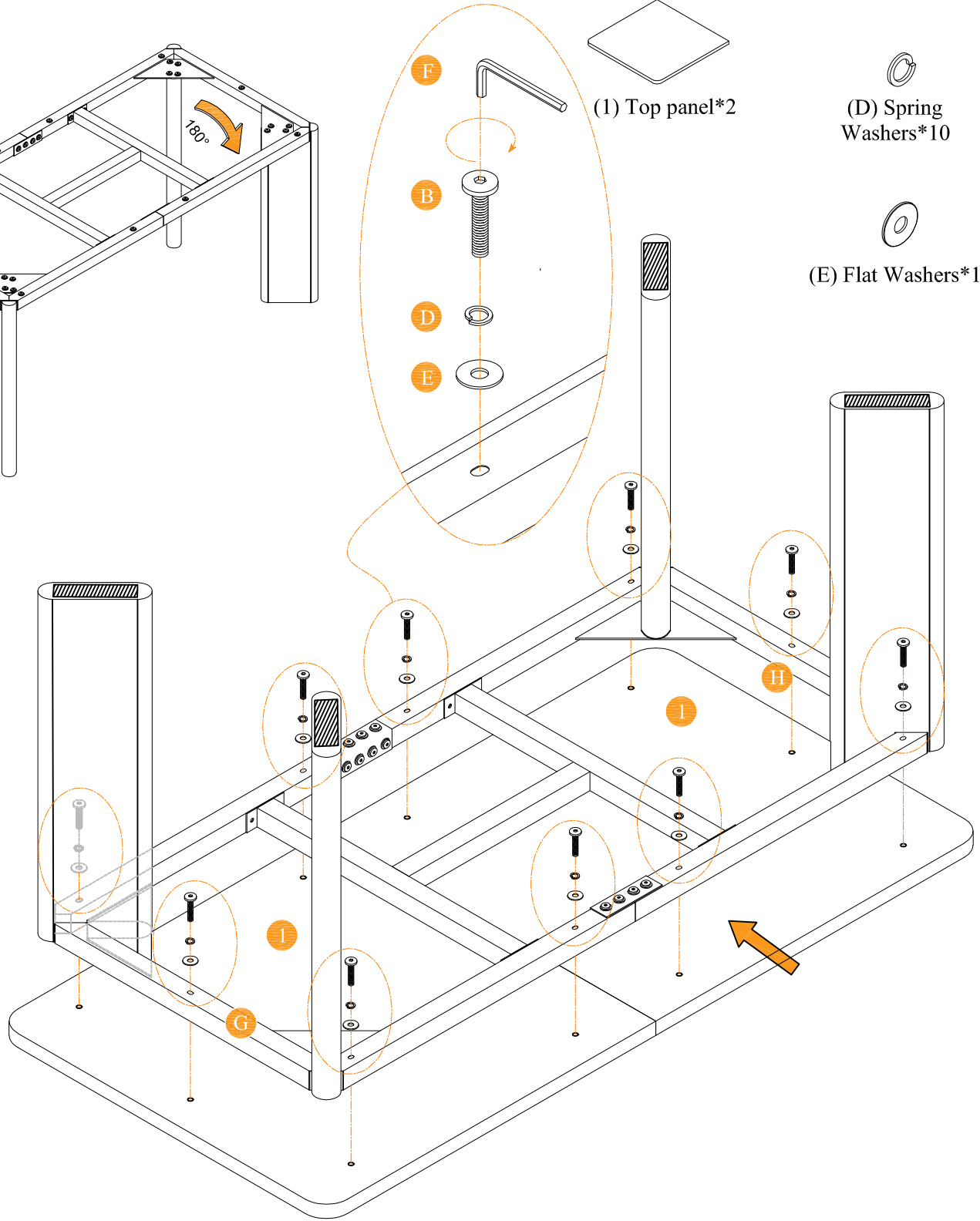
(B) Hex Head Screw M6X55mm *10
