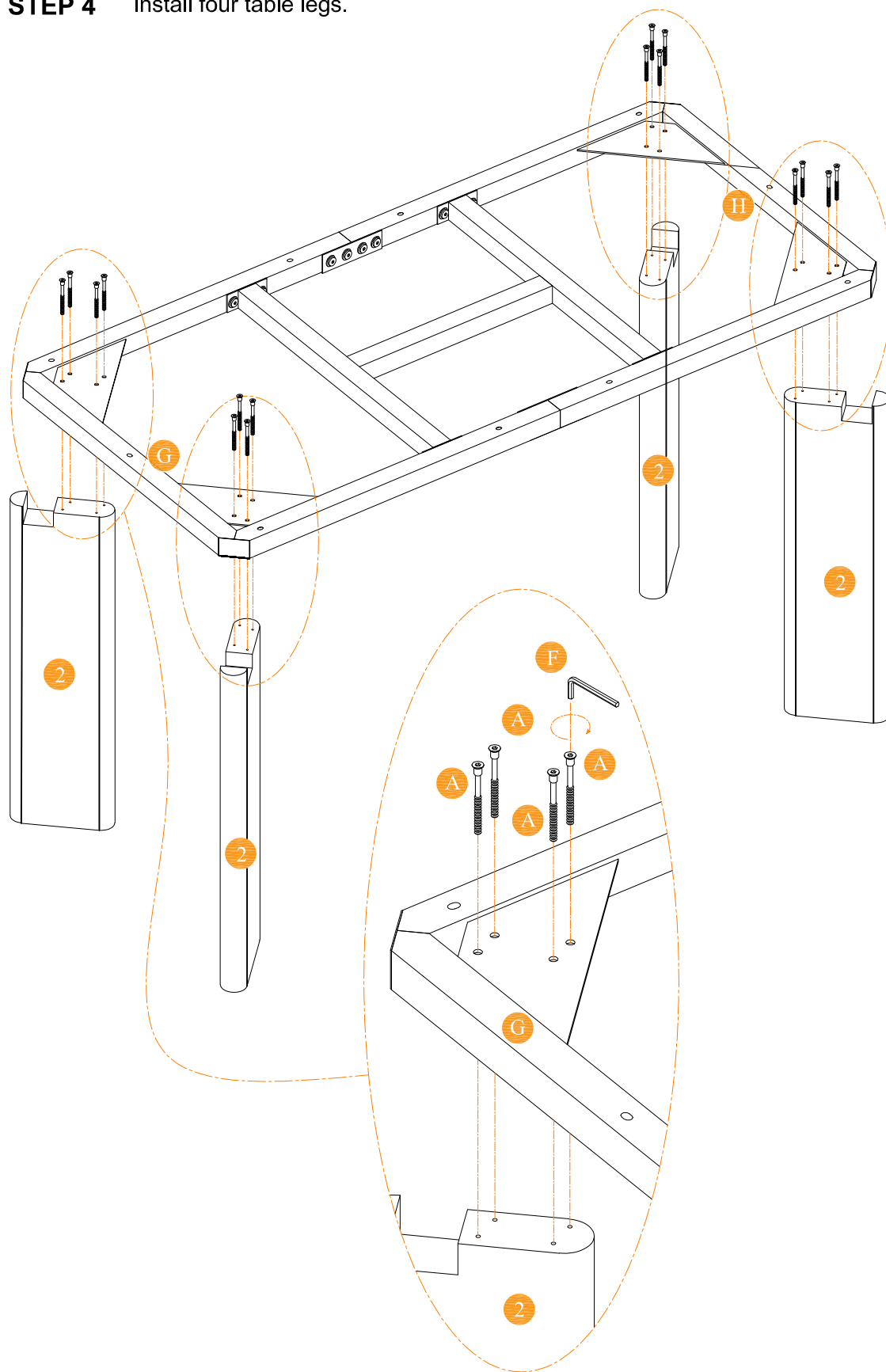
(A) Flat Head Screw M7x70mm*16
