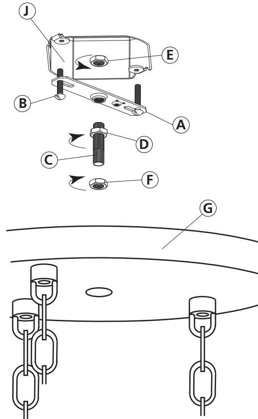
DRAWING 1 - MOUNTING
