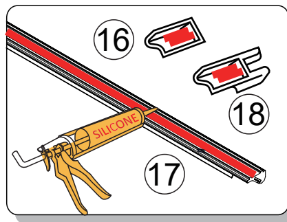
2. Apply glass sealant
