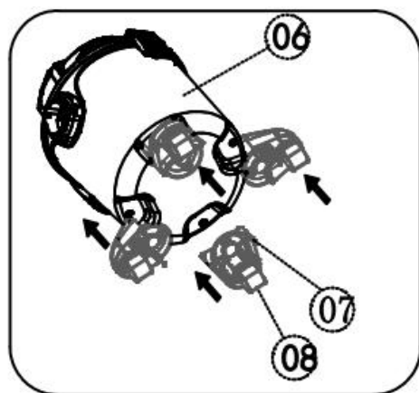
Wheels' assembly
