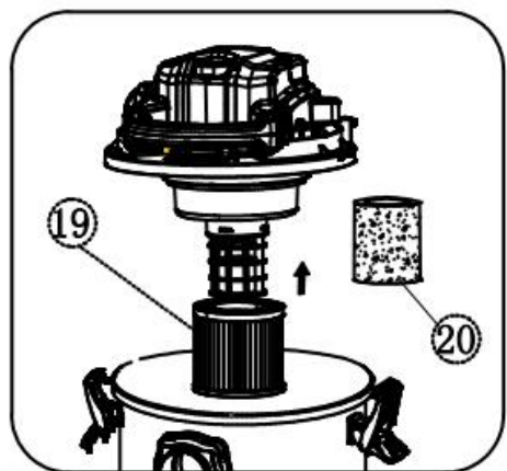
Sponge filter assembly for wet usage cleaning Function
