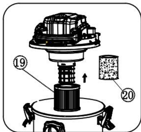
HEPA filter assembly for dry usage
