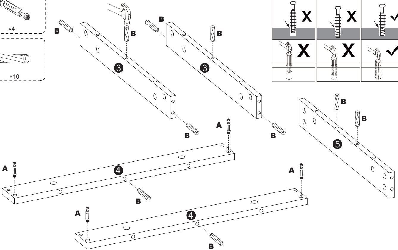
Installation method of three in one bolt
