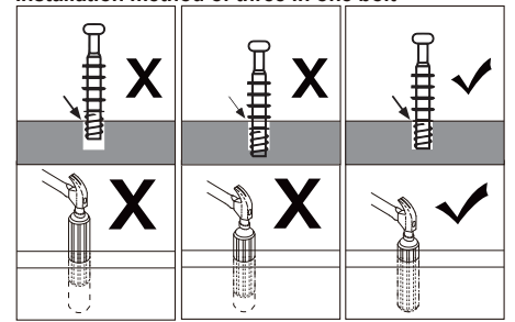
Installation method of three in one bolt
