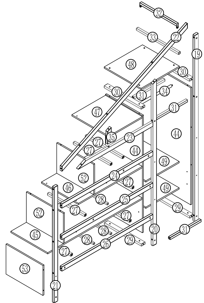
Stairs part view
