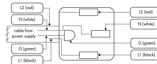
Four-Wire Connection Receptacle NEMA 14-50R
