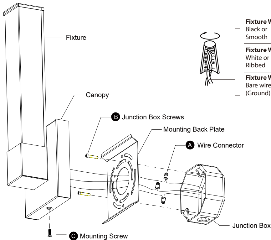
Fig.2 Wiring
