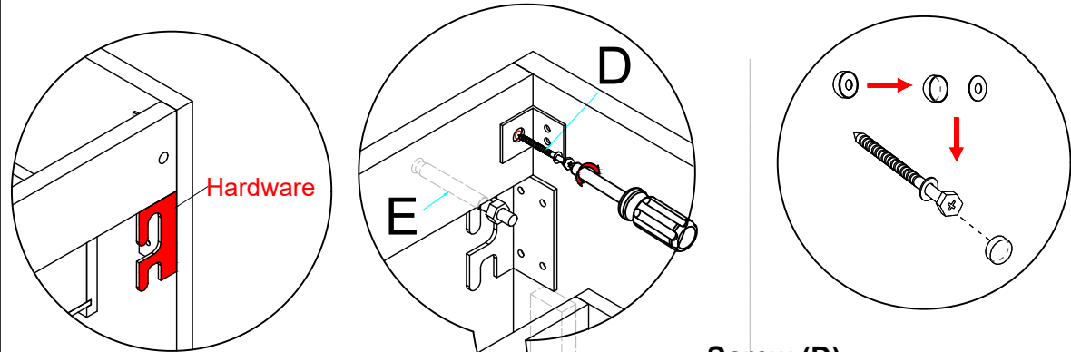
Screw (D): M5 x 50mm long (2pcs)
