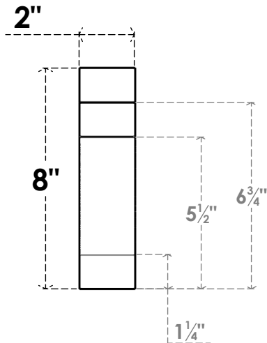
FRONT PROFILE
