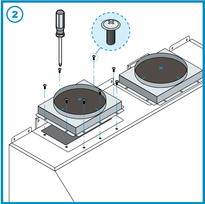
(Fig 2) Fasten on 10" - Ø Transition on to the top exhaust of range hood using M4-4mm (Big Head) screws.
