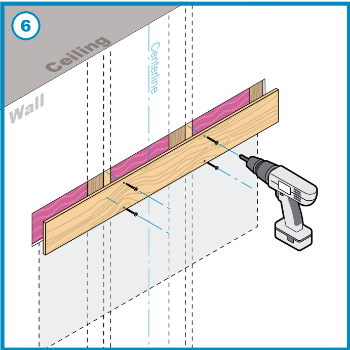
(Fig 6) Screw on plywood to the exposed studs (woodscrews not included). The inserted plywood should be the same depth as the drywall slab it is replacing.
