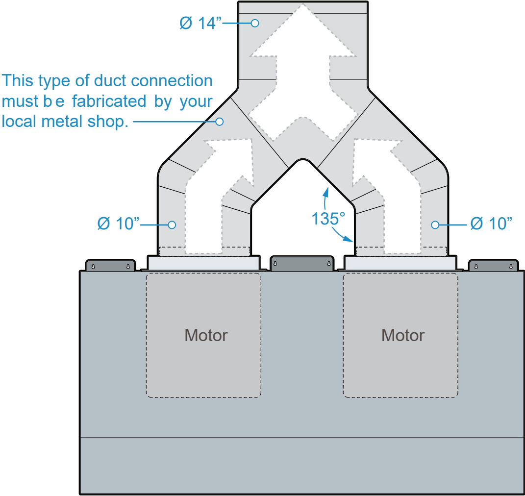
FRONT VIEW
