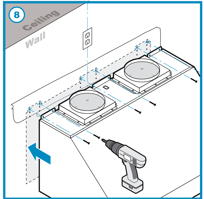
(Fig 8) Use woodscrews (not included) to screw onto the area of the plywood brace based on your measurements already established.
