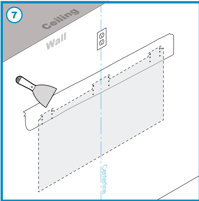
(Fig 7) Apply spackle in between spaces of the plywood and drywall seamlessly. Sand down any rough spackle to smooth out. Paint area if required.
