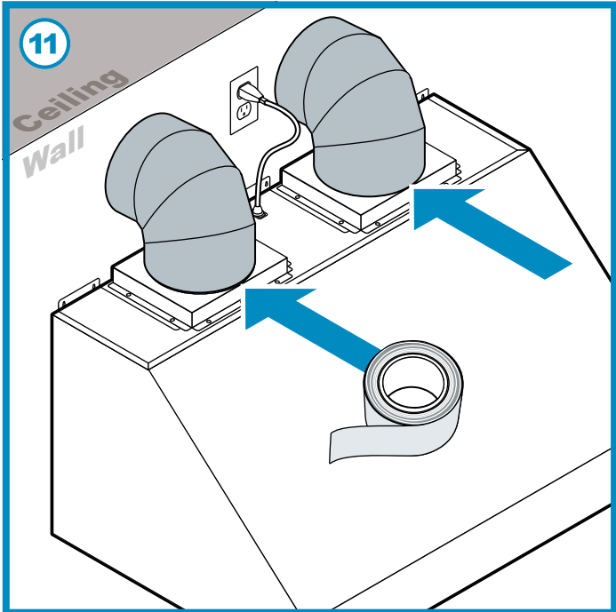
Fig 11) Use aluminum foil tape to make all joints secure and air tight.
