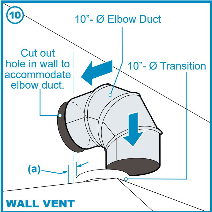
Fig 10 (a) Distance from wall to transition circumference edge for 10" - Ø Transition will be 1/2".
