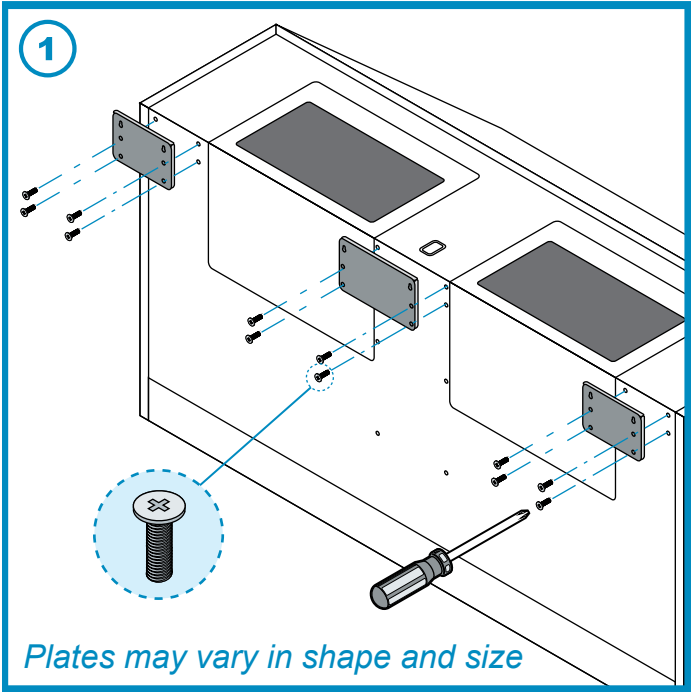
(Fig 1) Fasten installation plates using M4-4mm screws (countersink) on to the back of the range hood.
