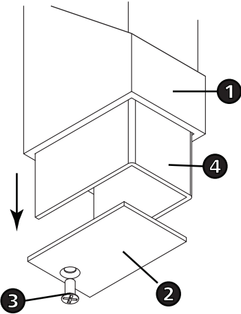
DRAWING 2 - Lens removal
