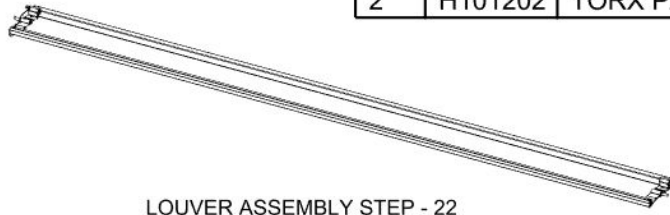
LOUVER ASSEMBLY STEP - 22 (x4)
