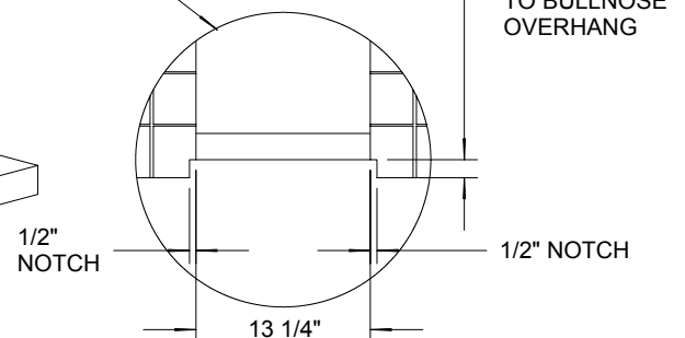
BULLNOSE NOTCH DETAIL
