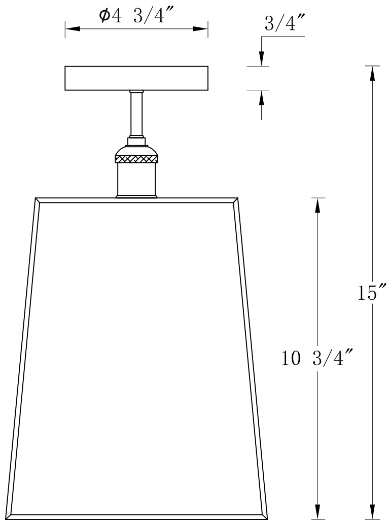
FRONT VIEW
