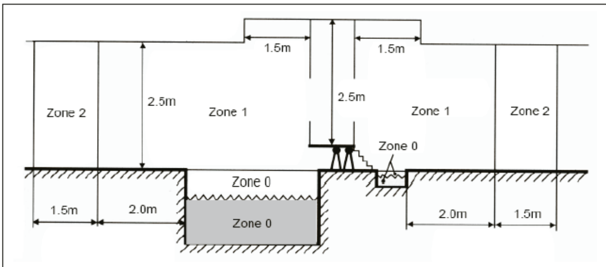
Above figure: Zone dimensions of swimming pools and paddling pools
