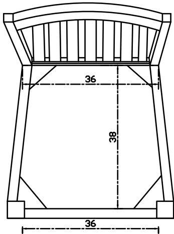
TOP VIEW (FRAME)
