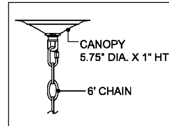
CANOPY DETAIL
