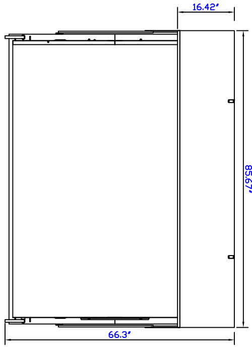
open Top view
