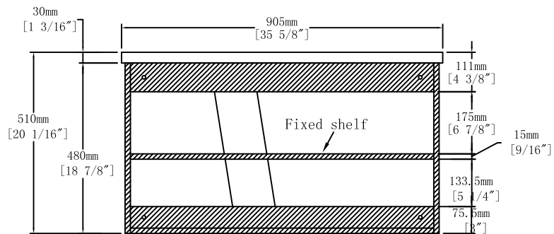
Back View
