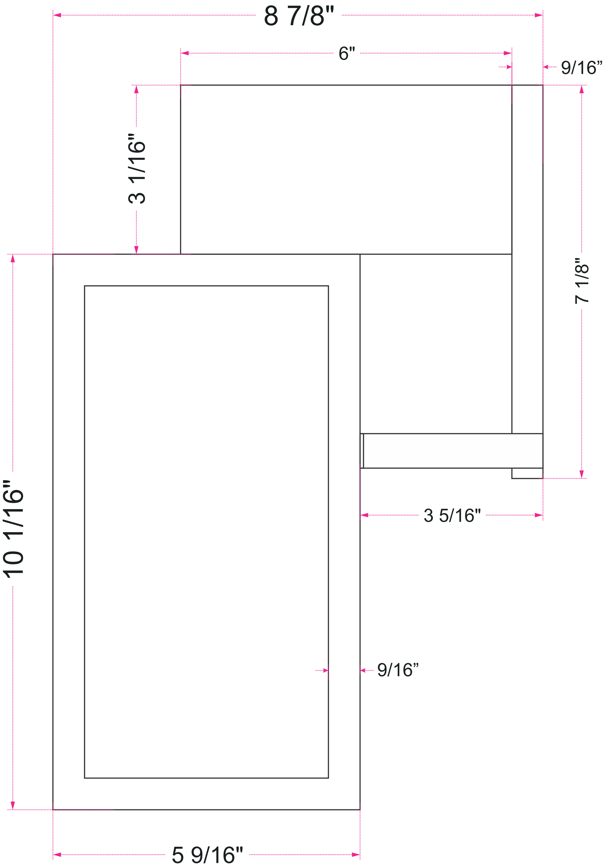
Side View
