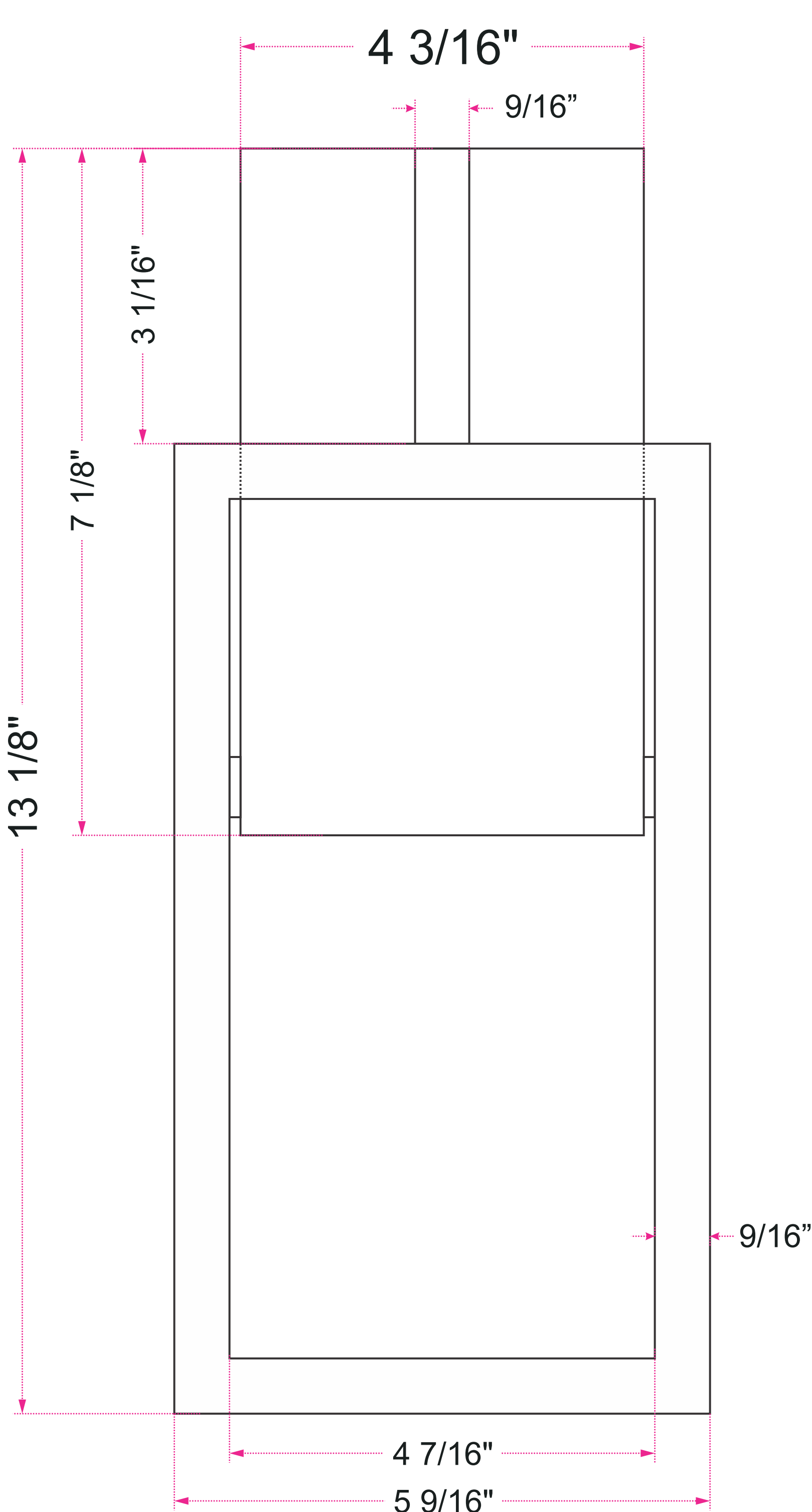
Front View
