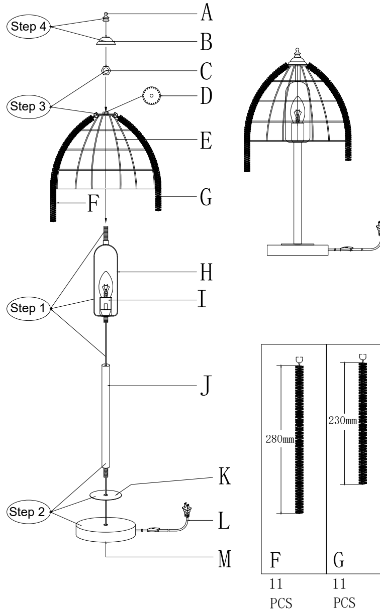
Lighting structure explosion diagram
