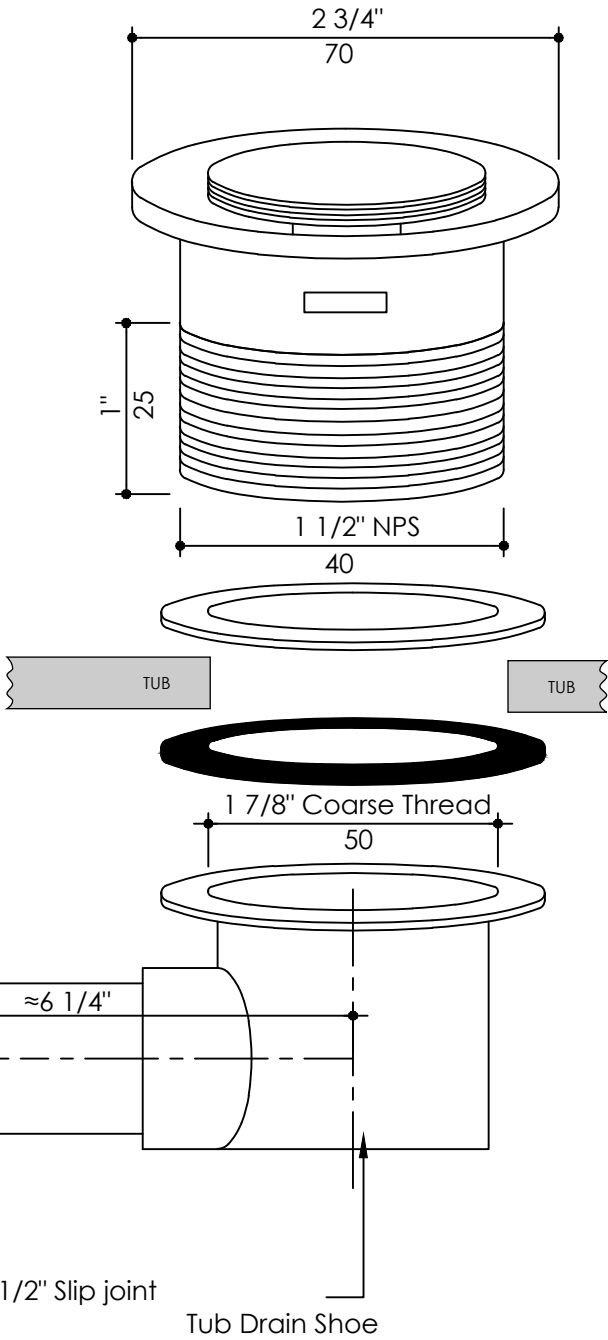
Tub shoe and P-trap connections. Suggested pipe is 1-1/2" diam
