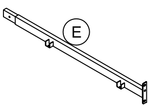
Side Rail 02 T943180 X 2
