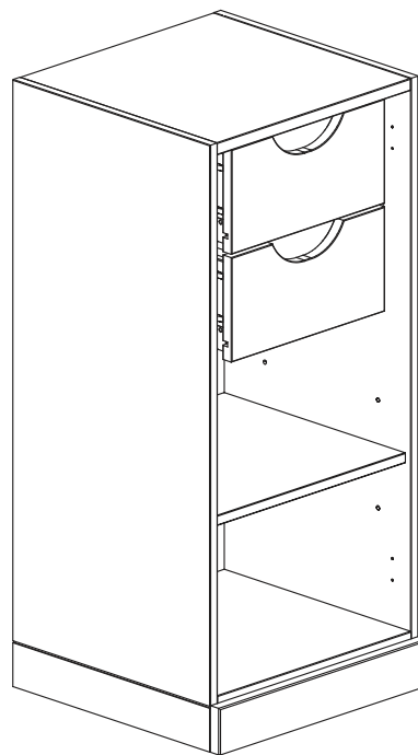
16.5" Unit + Drawers
