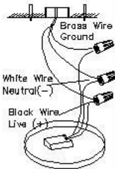
Connect the wires
