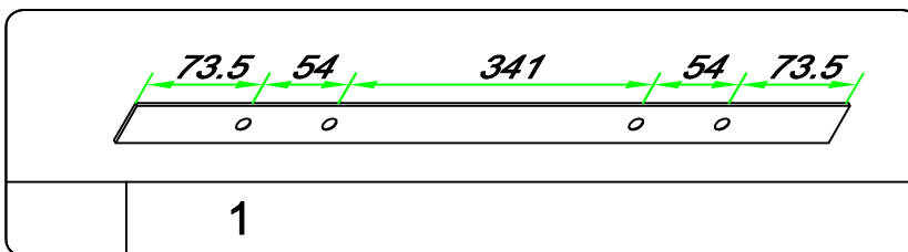
Installation template
