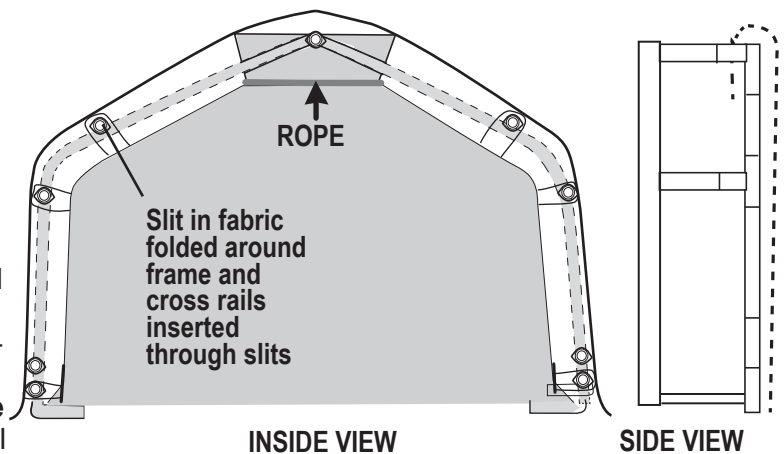
DETAIL I
