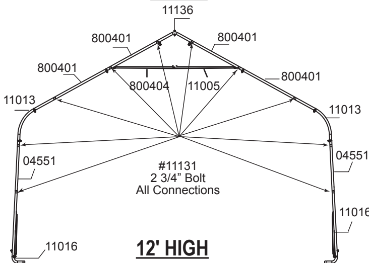
DETAIL B End Ribs
