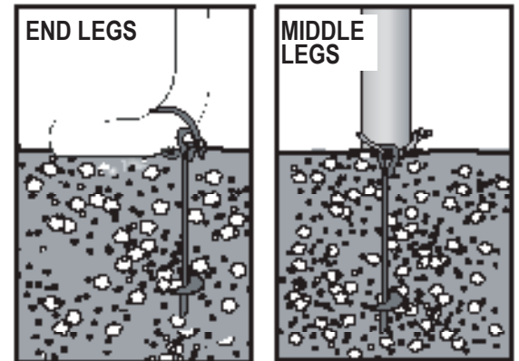
DETAIL H
