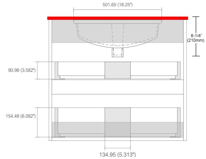
. DRAWER PANELS
