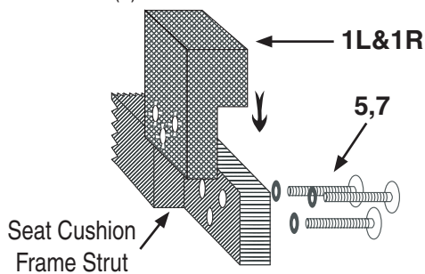
Fig.3: Insert Rear Leg (1) next to Seat Cushion (3) frame.
