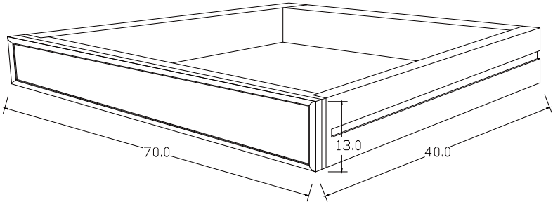
DETAIL DRAWER
