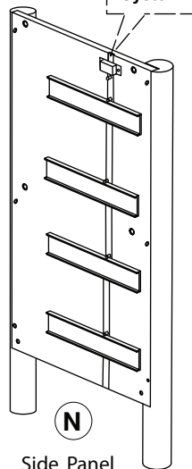
N Side Panel (Right Hand) x 1
