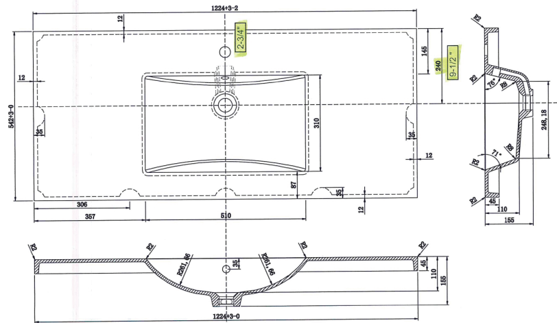
SINK DETAIL
