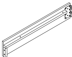
18 (1041.5x170x56mm) x 2
