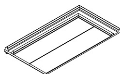
2 (858x667x62mm) x 1
