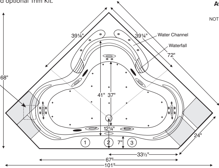
Numbered areas on tub deck represent possible locations to install cleaning systems, faucets and other fixtures. Shown with Air Massage and Ultra Whirlpool Package.
