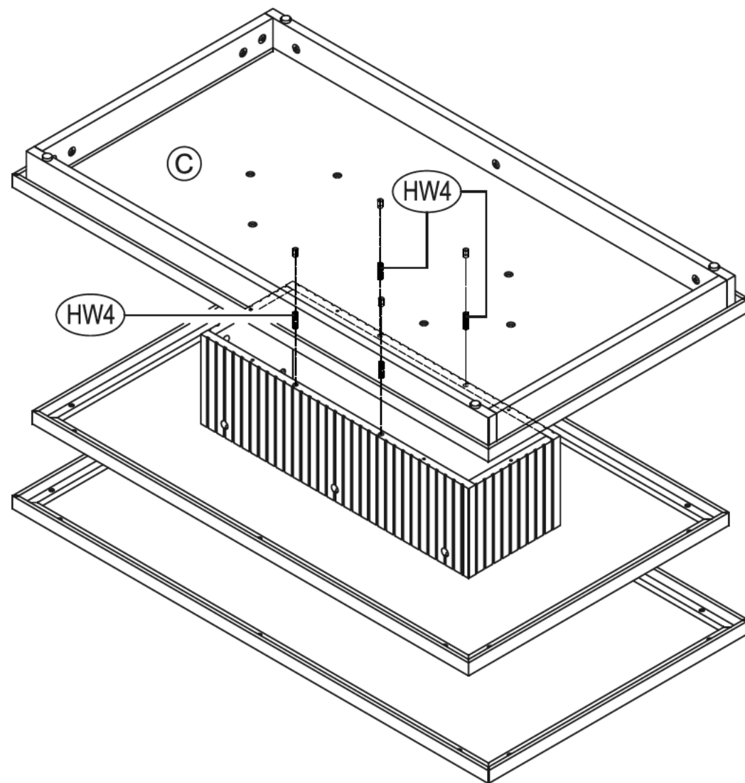
STEP 9 ATTACH BOTTOM PANEL (C) TO UNIT USING 28MM DOWELS (HW4).
