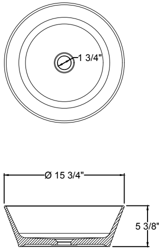
KCV-205 15 3/4" x 5 3/8"
