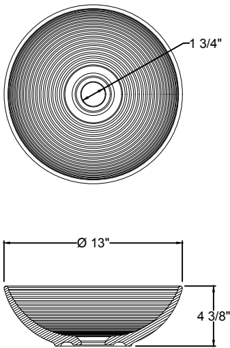
KCV-204 13" x 4 3/8"
