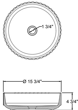
KCV-201 15 3/4" x 4 3/4"
