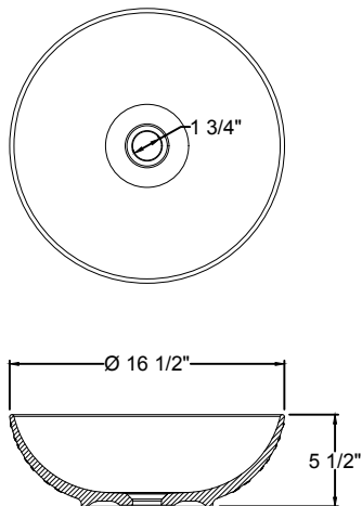
KCV-200 16 1/2" x 5 1/2"
