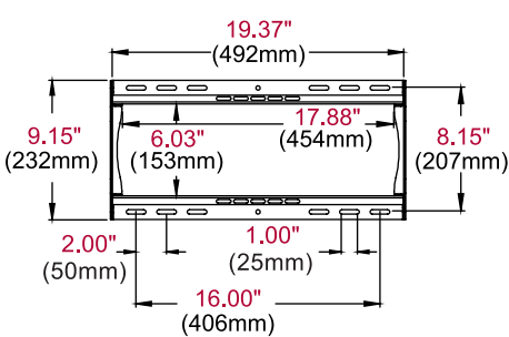
WALL PLATE
