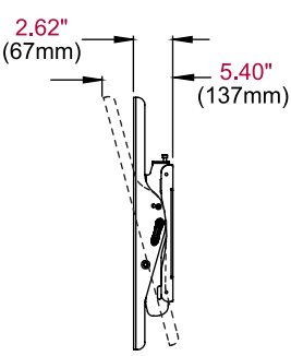
SIDE VIEW +15/-5° TILT
