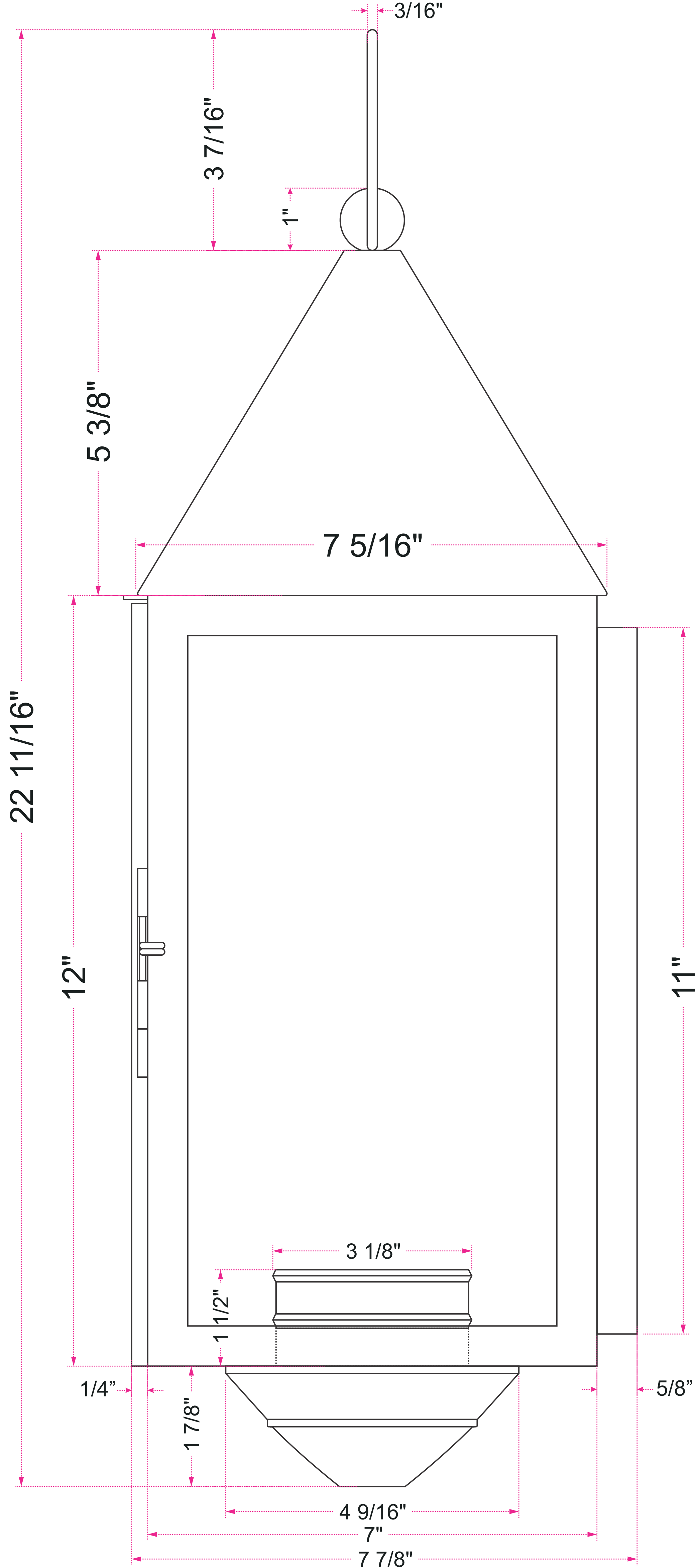
Side View
