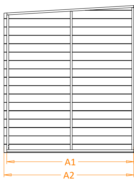
BLANK GABLE - RH x1 PER SHED
