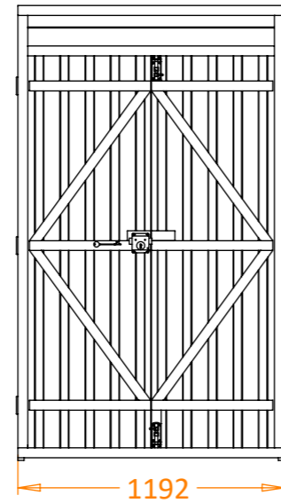
DOOR SIDE x1 PER SHED
