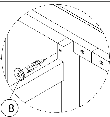
Center frame
