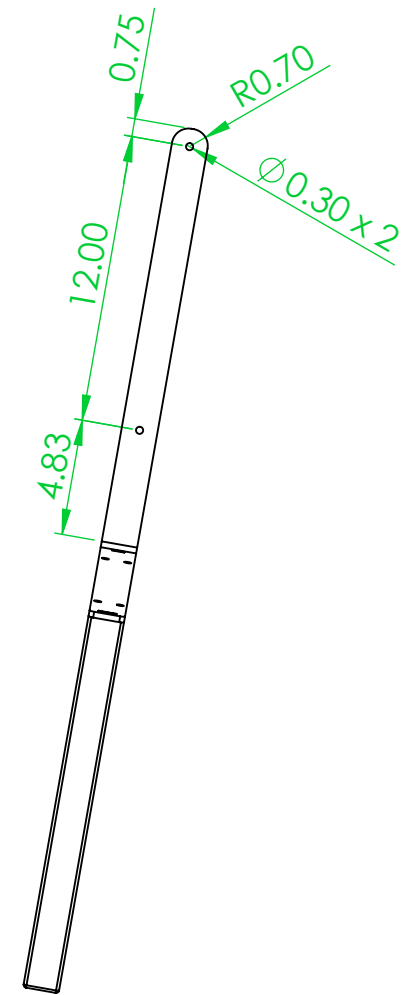
VIEW C
