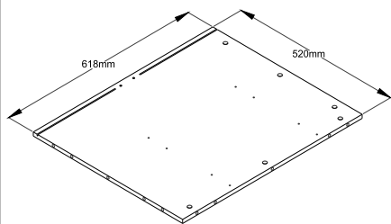
Small Side Panel-R Qty:1
