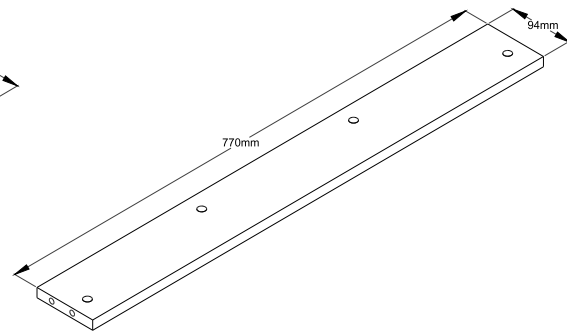
Bottom Rear Support Panel Qty:1
