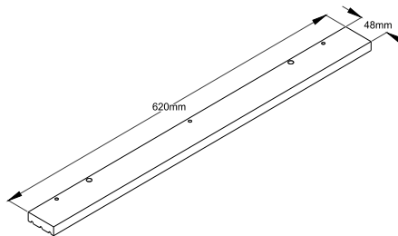
Front vertical bar Panel Qty:2
