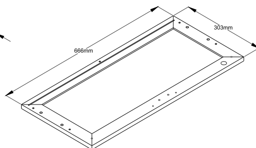
Drawer Front Panel Qty:1
