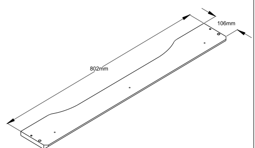
Lower Front Support Panel Qty:1
